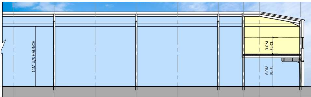
TYPICAL BUILDING SECTION B-B
